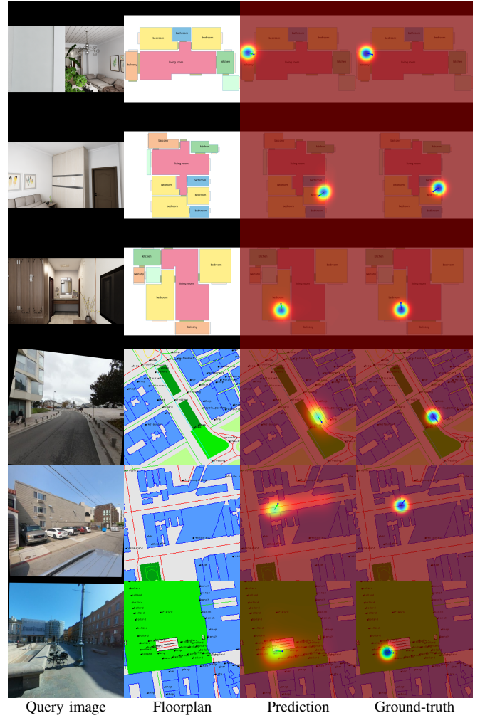
Fig. 4: Qualitative results of SLoFT. Our model is evaluated on the official Structured3D test set of areas never seen during training , and on the MGL validation set for fair comparison with previous works [11]. The results show that our model excels at understanding both the semantic context from the query image (rows 1,4,6) and implicitly reasoning about the geometry of walls and buildings (row 2,3,5), without explicit geometric supervision.
